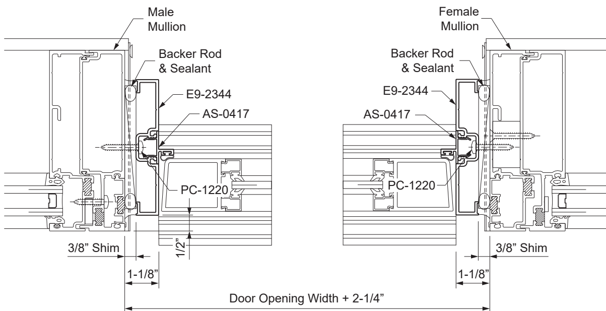
Detail 76
