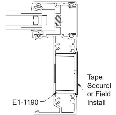
Detail 61
