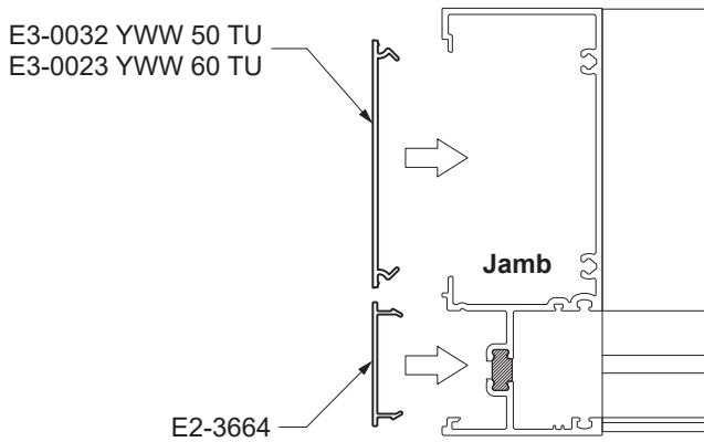
Detail 21
