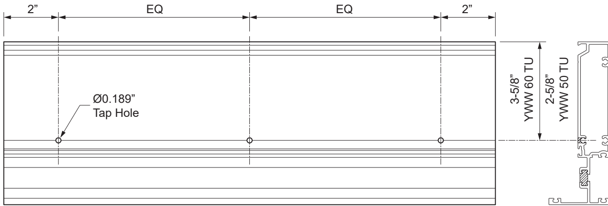
Detail 6
