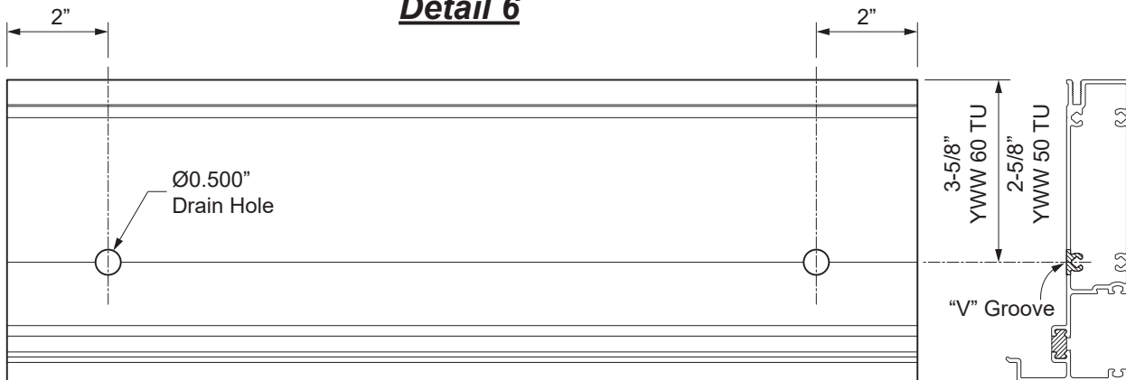
Detail 6
