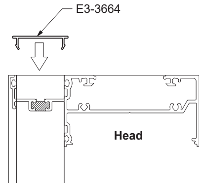
Detail 22 Outside Glazing Shown Inside Glazing Similar
