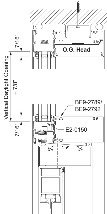
Detail 77
