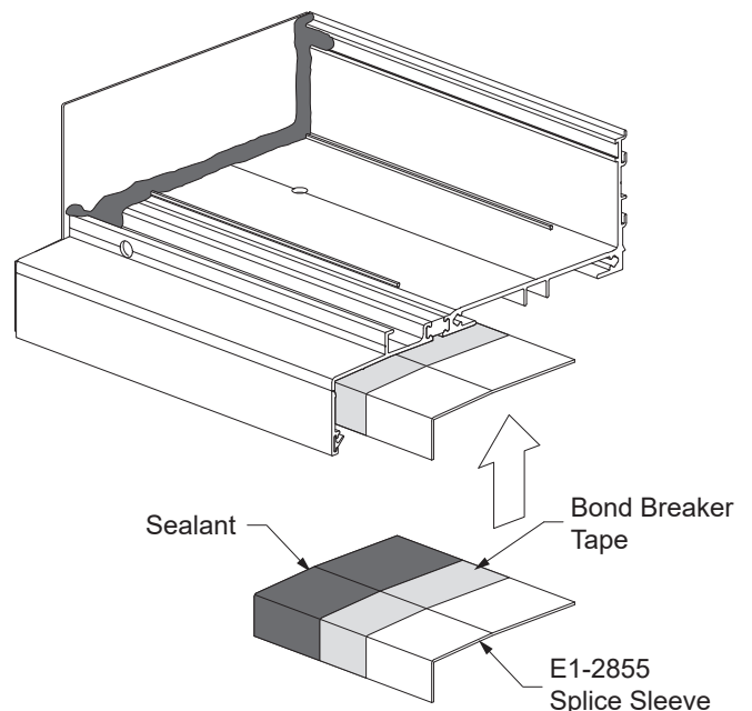
Detail 56
