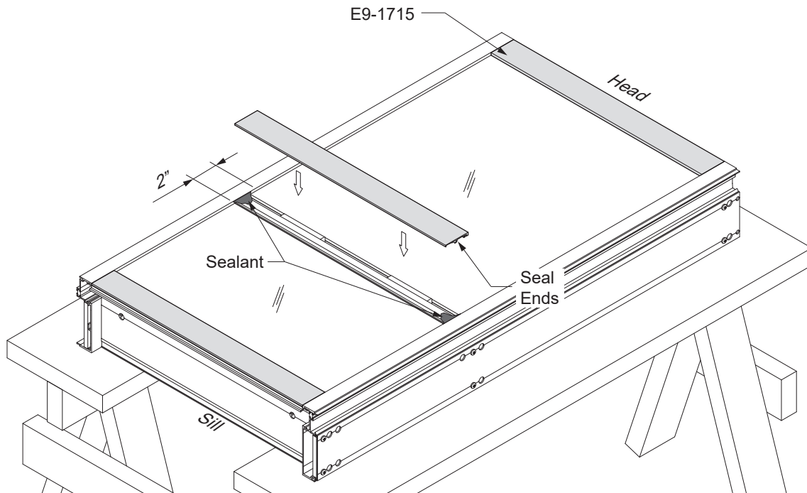
Detail 33
