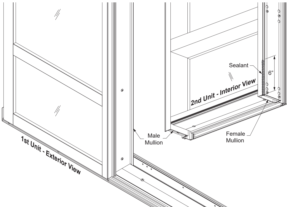
Detail 65
