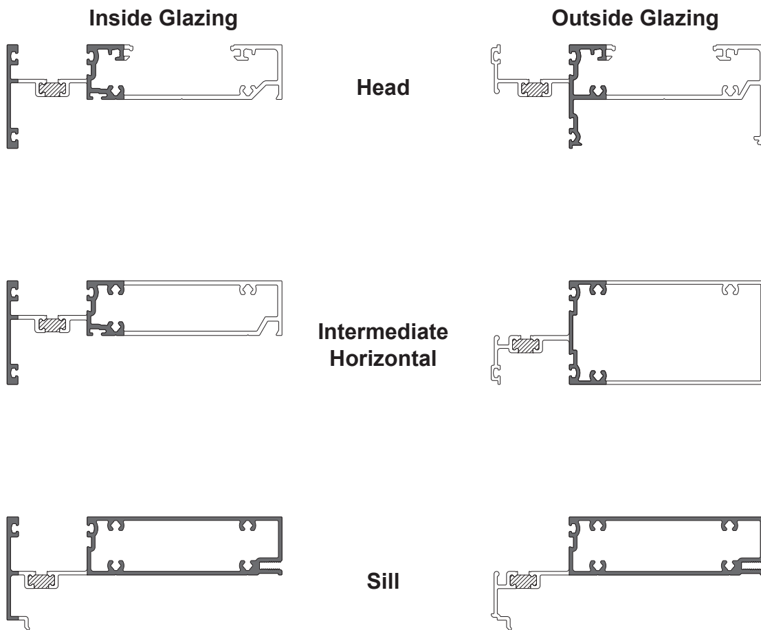
Detail 15
