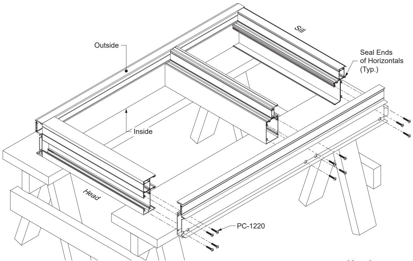
Detail 17 Outside Glazing shown, Inside Glazing Similar
