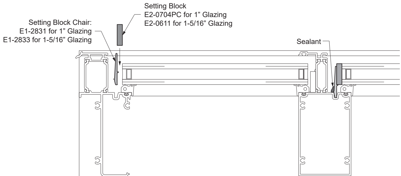
Detail 35 Outside Glazing Shown, Inside Glazing Similar
