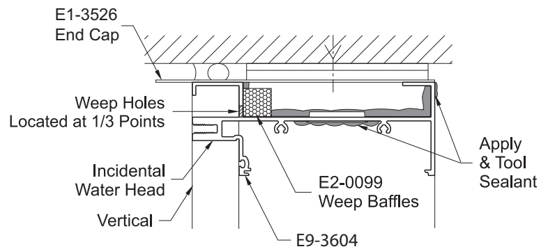
Detail 22
