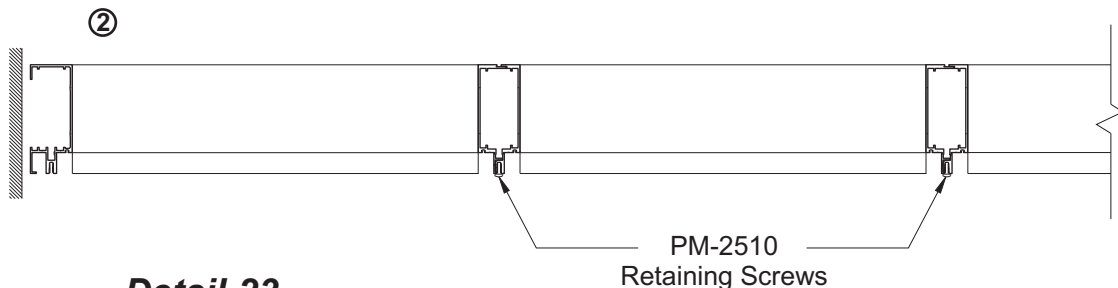
Detail 23
