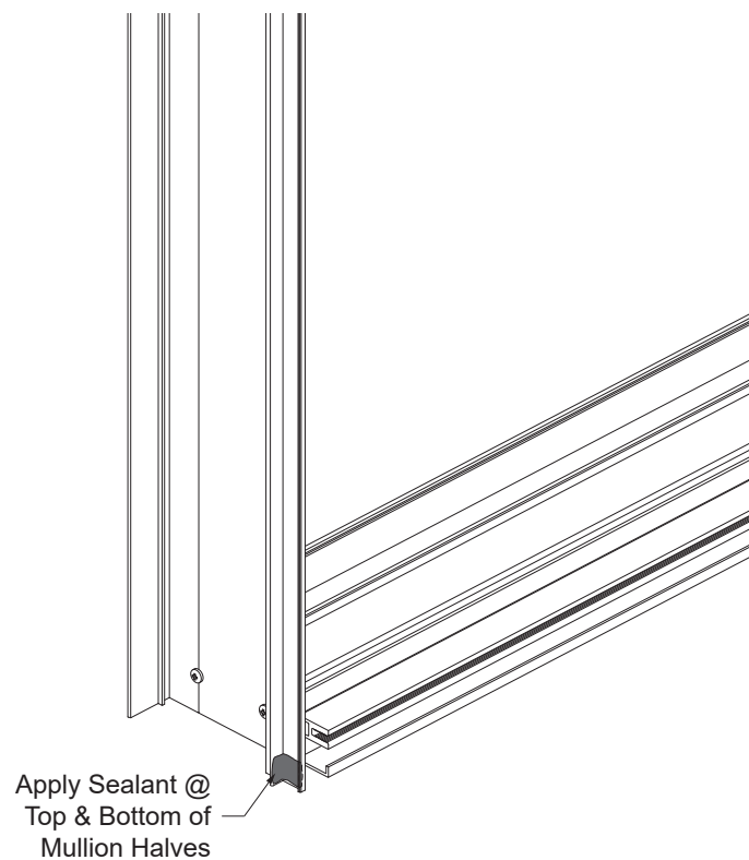
Detail 24 Bottom Shown, Top Similar
