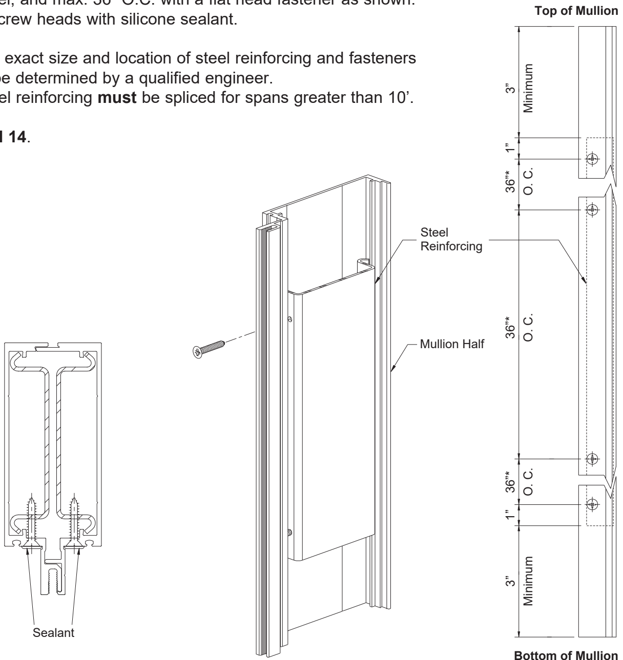
Detail 14
