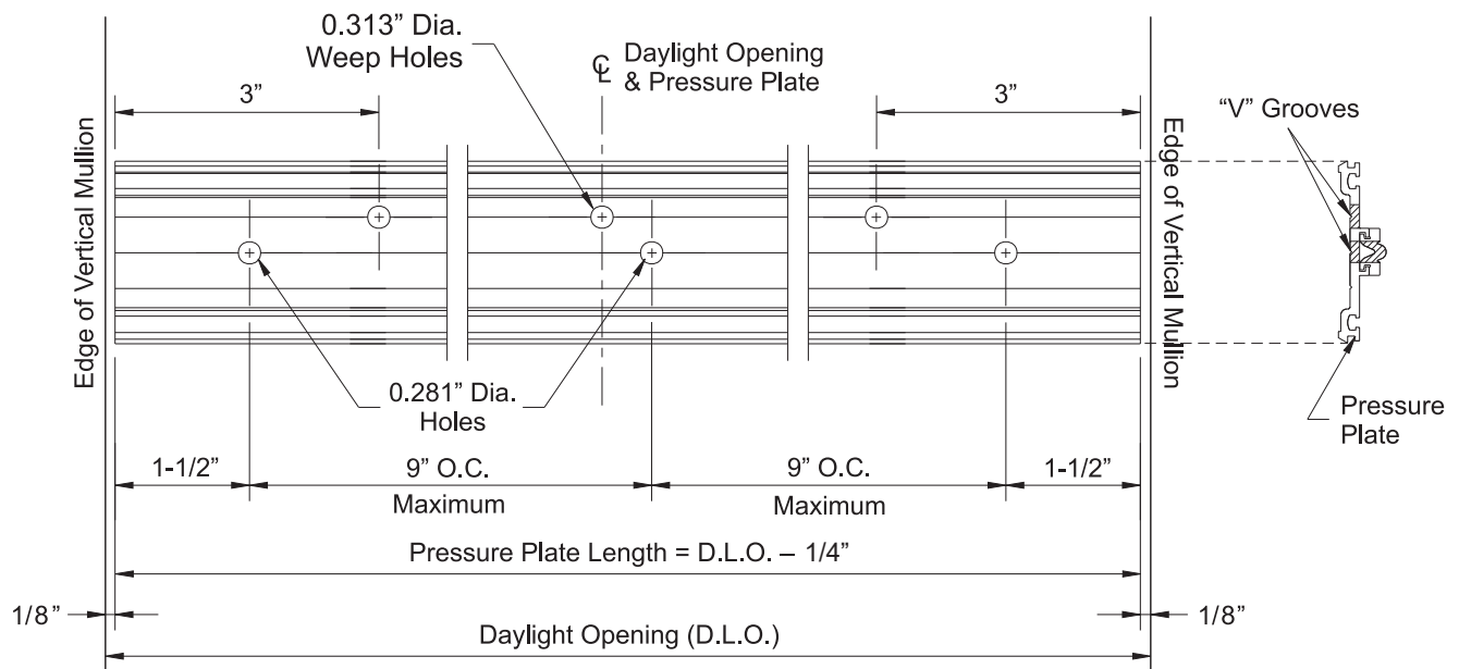
Detail 7
