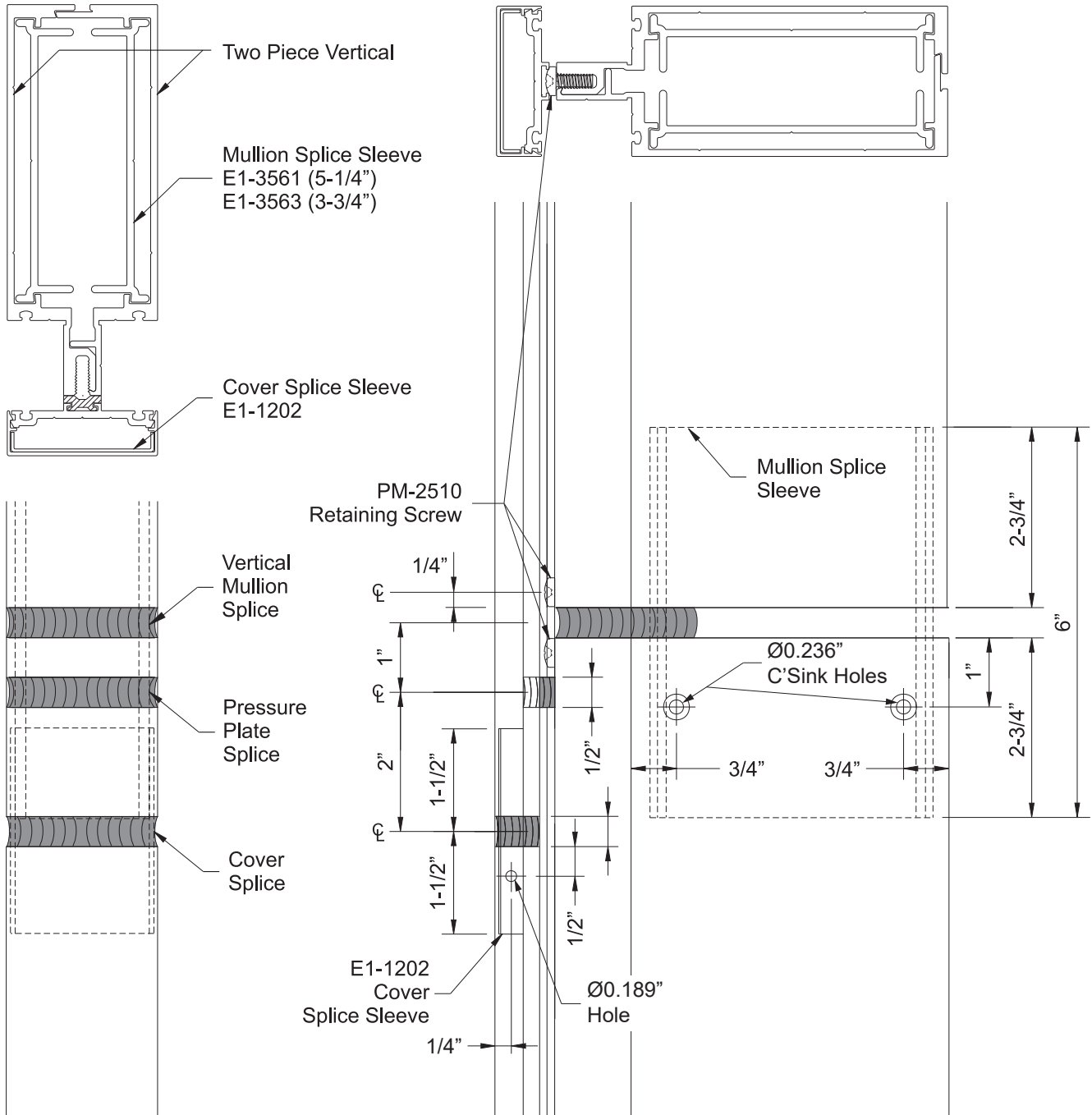
Detail 16
