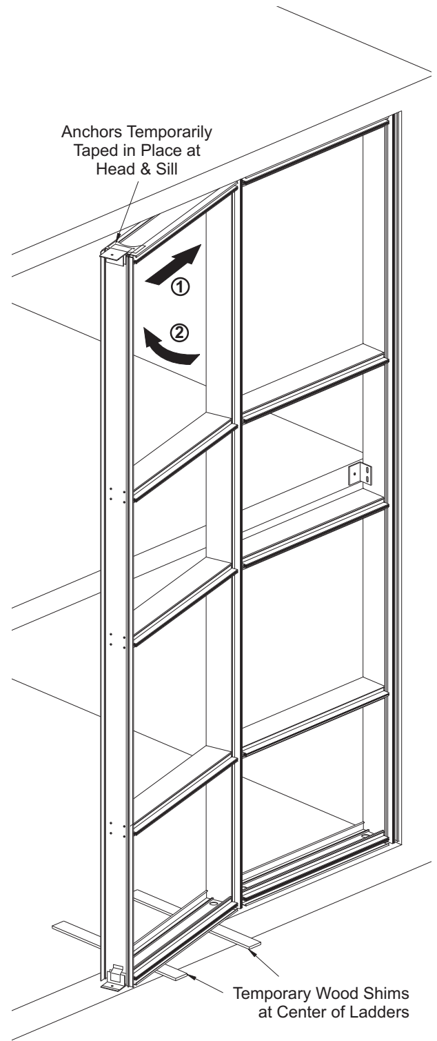
Detail 25
