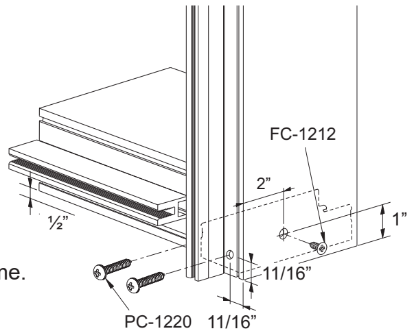
Detail 30
