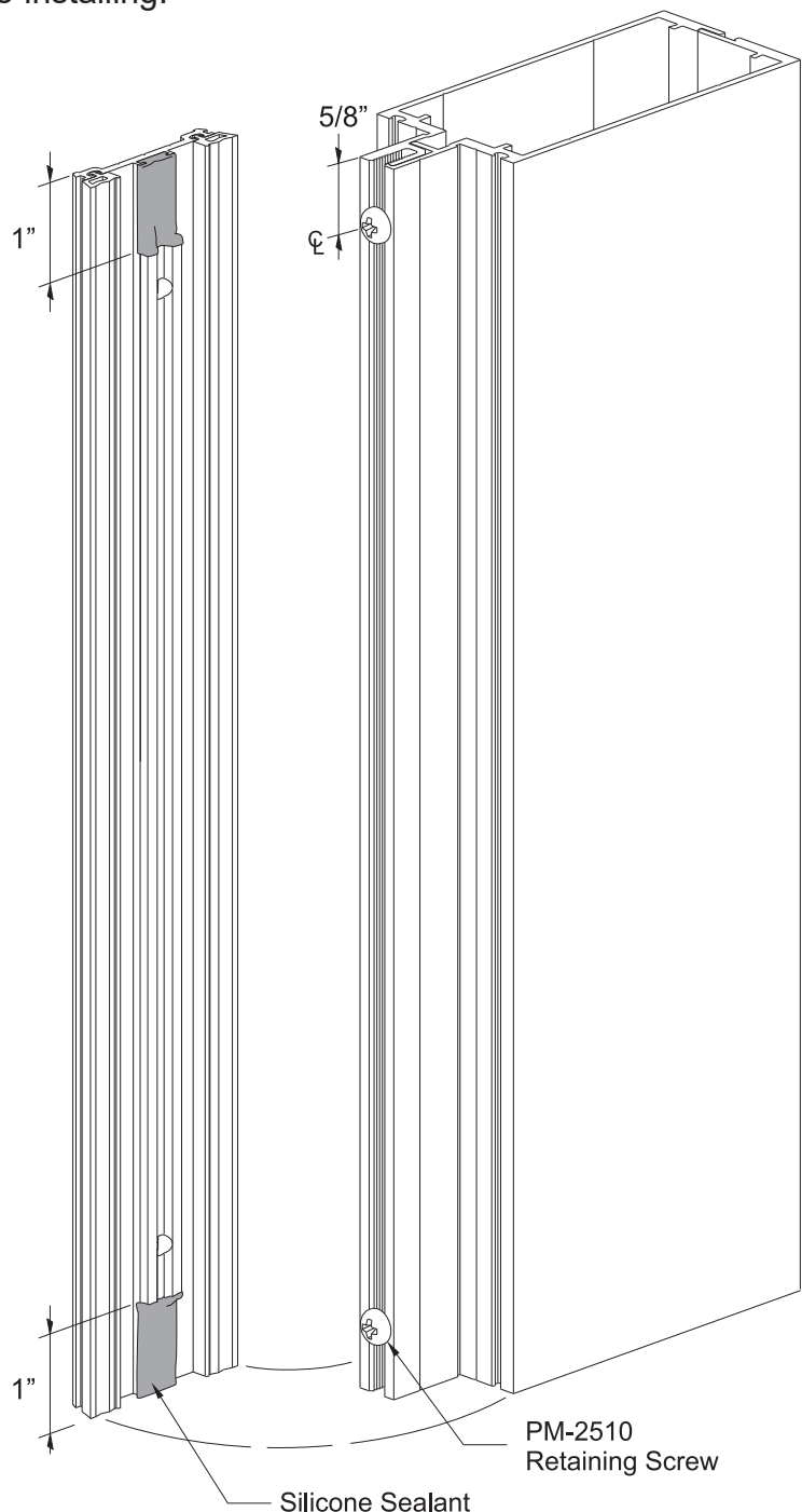
Detail 37
