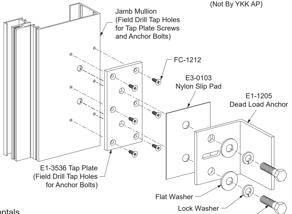
Detail 28A
