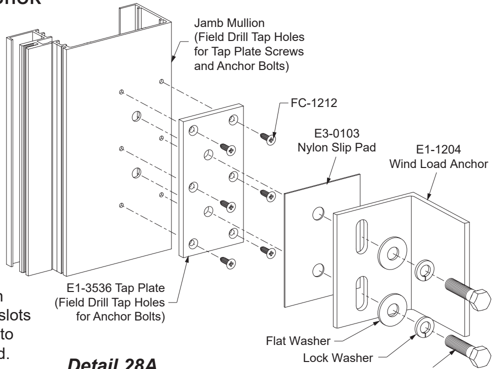
Detail 28A
