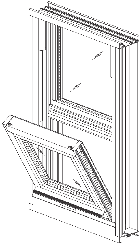
SINGLE HUNG
