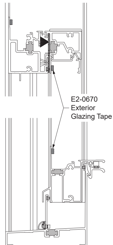
DETAIL 6
